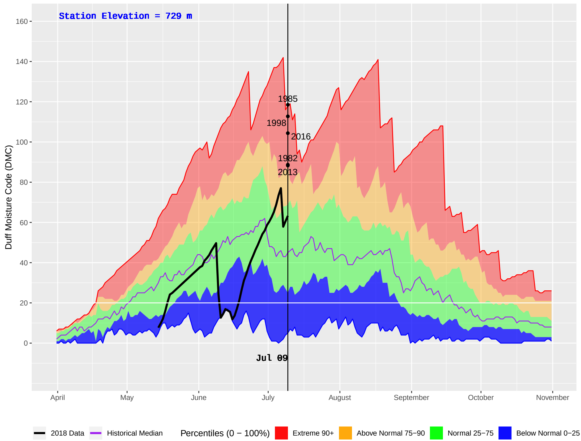
ATLIN (111) : Historical (1977–2016) and Current (2018) Daily Duff Moisture Code (DMC)
