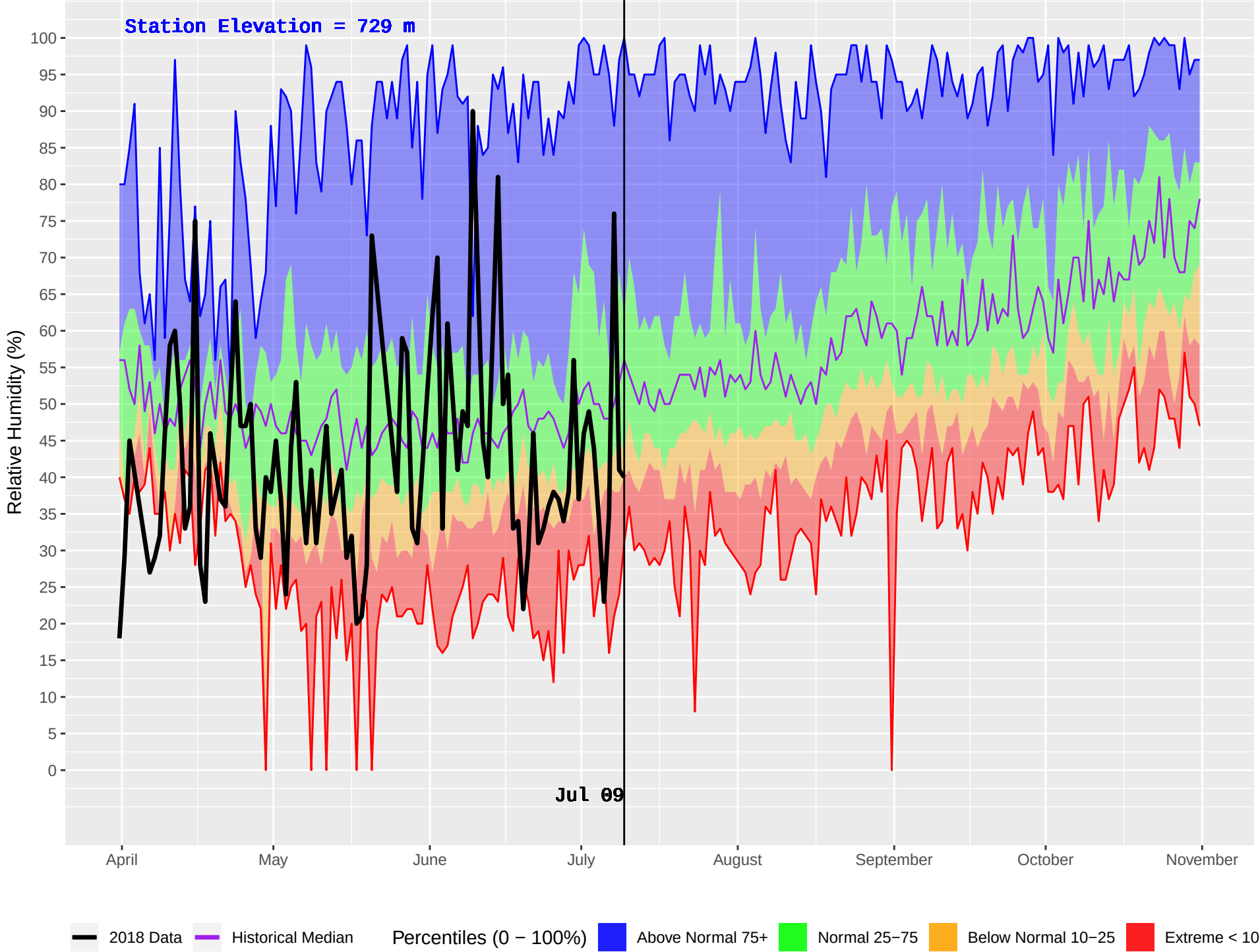
ATLIN (111) : Historical (1977–2016) and Current (2018) Daily Relative Humidity
