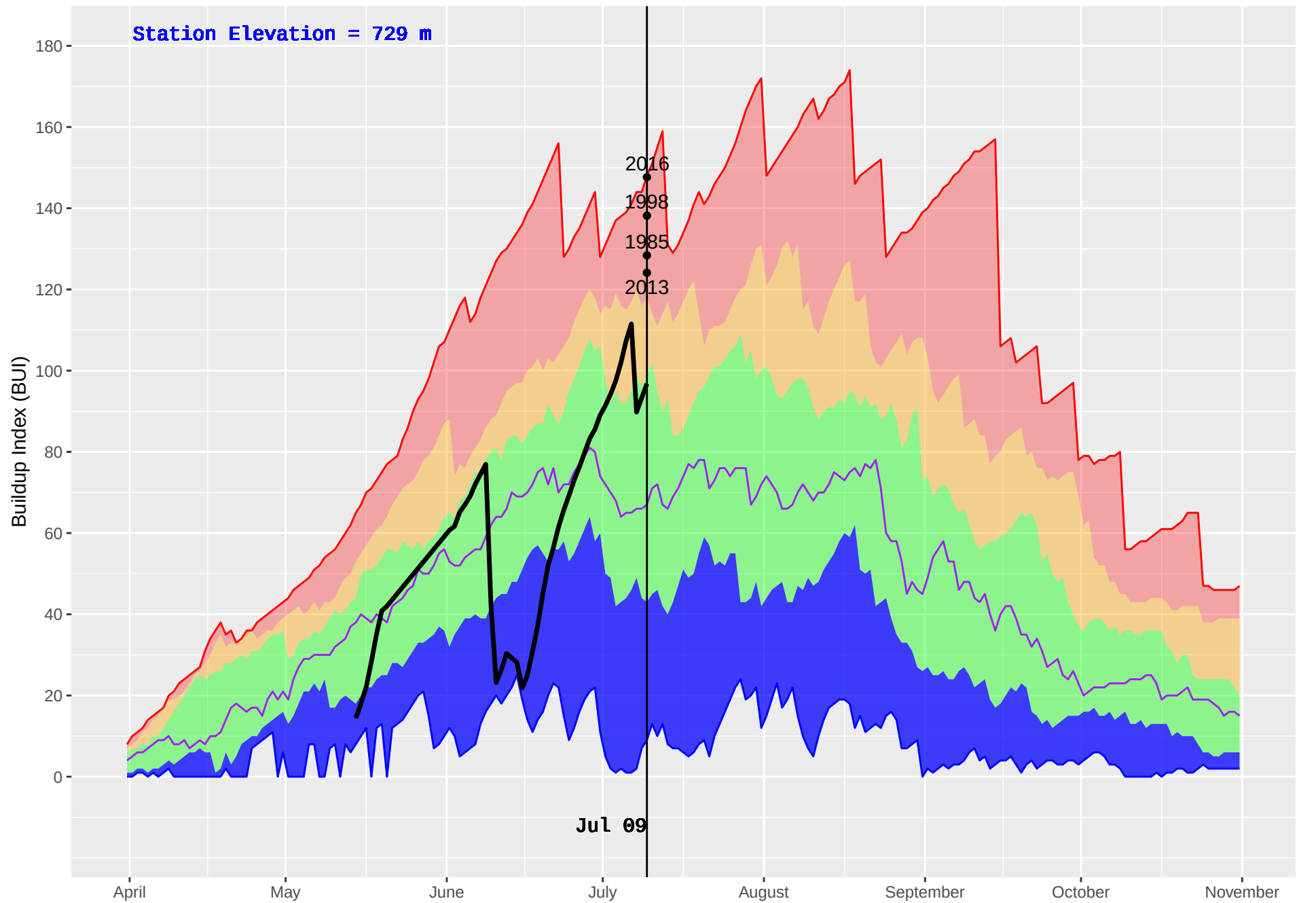
ATLIN (111) : Historical (1977–2016) and Current (2018) Daily Buildup Index (BUI)
